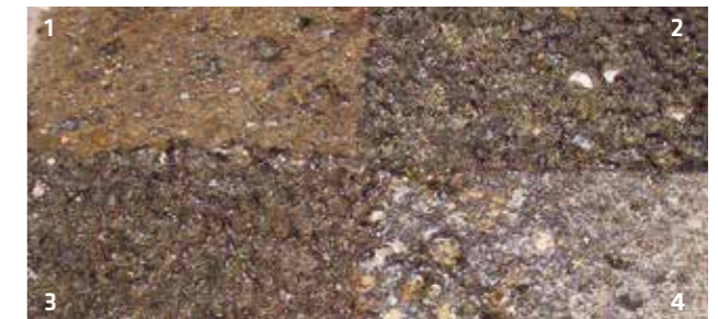
Fire exposure trials for concrete containing various aggregates. Surface spalling and sintering, and a range of temperature developments at differing depths can thereby be compared.
