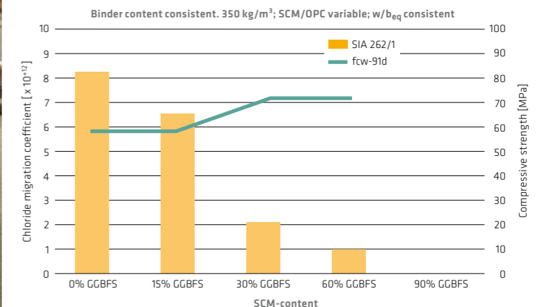
Figure 7: Concrete tests according to SIA 262/1 Annex B (similar to NT BUILD 492)
