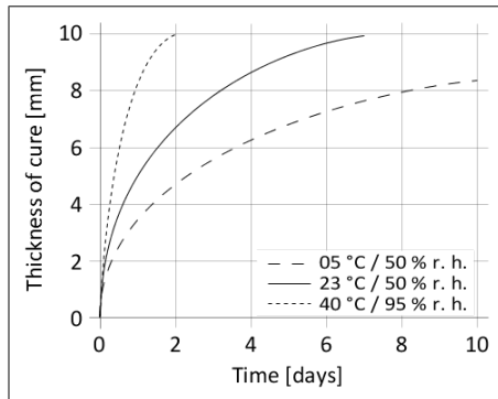
Diagram 1: Curing speed Sikasil® WS-300 EU
