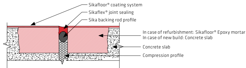
New build or refurbishment of a driveable movement joint
